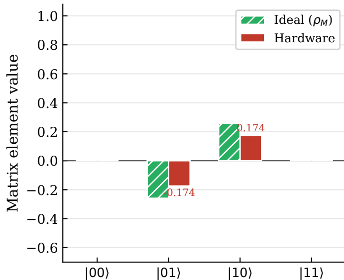
(f) \text{Im}(\rho_Y)
