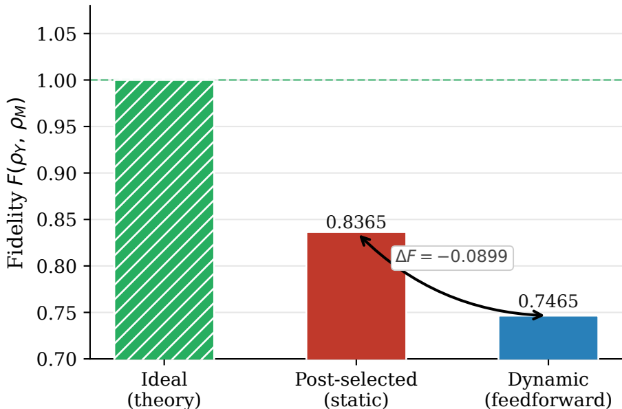
Output fidelity comparison (ibm_torino · 95% bootstrap CI)
