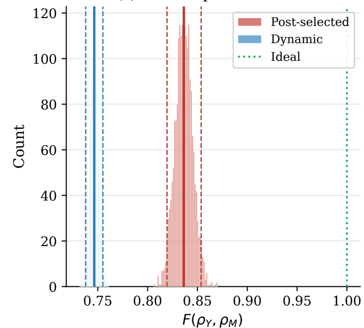
(c) Bootstrap distributions
