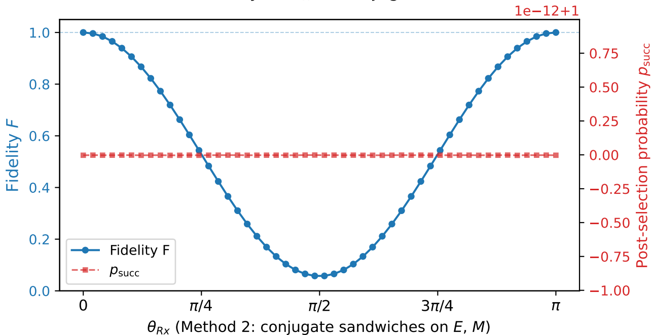
Method 2: Fidelity vs R_x(\theta) conjugate sandwiches
