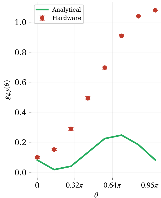
(c) g_{\phi\phi}(\theta) : hw vs analytical
