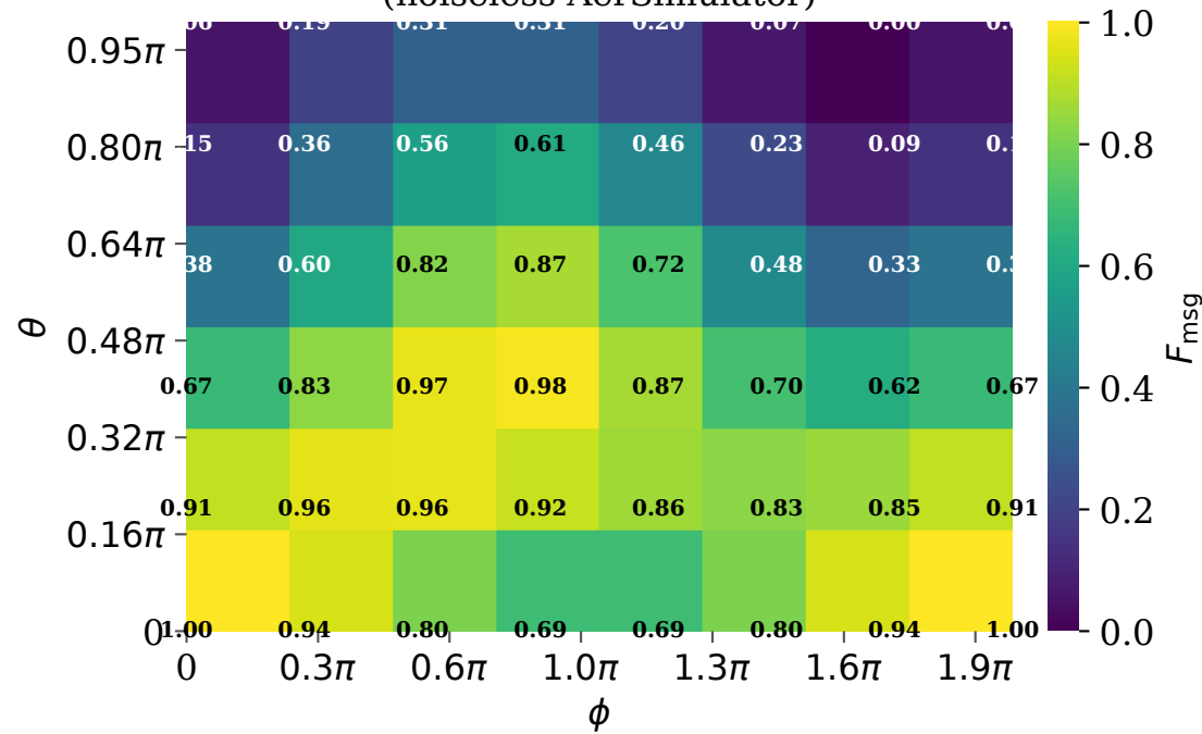
(a) Simulator F_{\text{msg}}(\theta, \phi) (noiseless AerSimulator)
