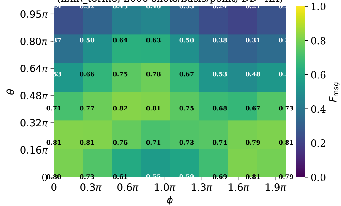
(b) Hardware F_{\text{msg}}(\theta, \phi) (ibm\_torino, 2000 shots/basis/point, DD=XX)
