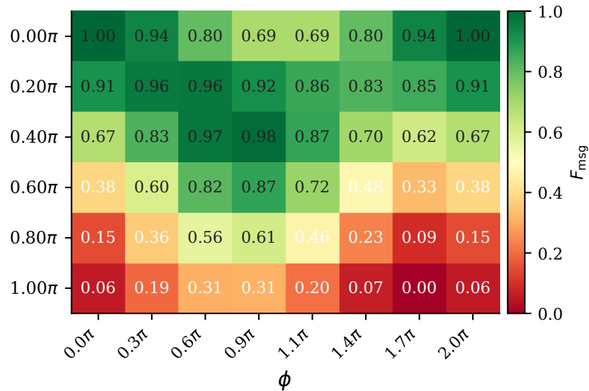
(a) Simulator F_{\text{msg}}(\theta, \phi) (noiseless)
