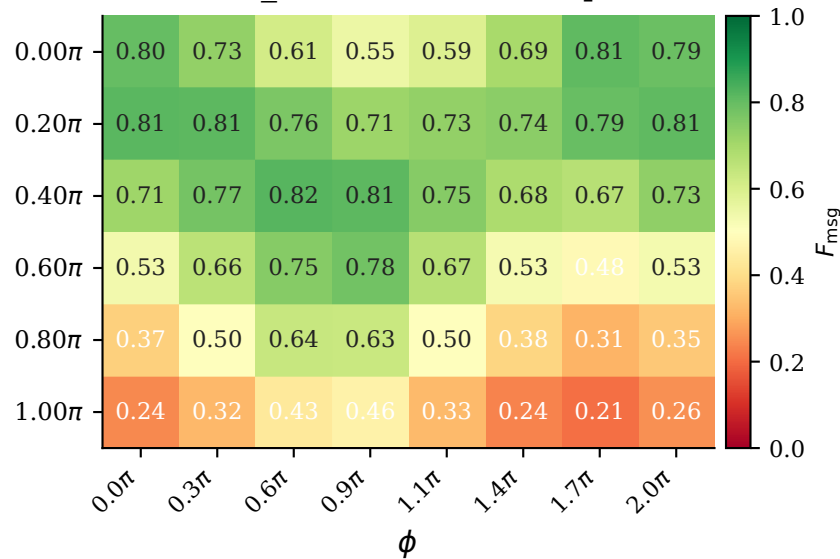
(b) Hardware F_{\text{msg}}(\theta, \phi) (ibm_torino, 2000 shots/pt)
