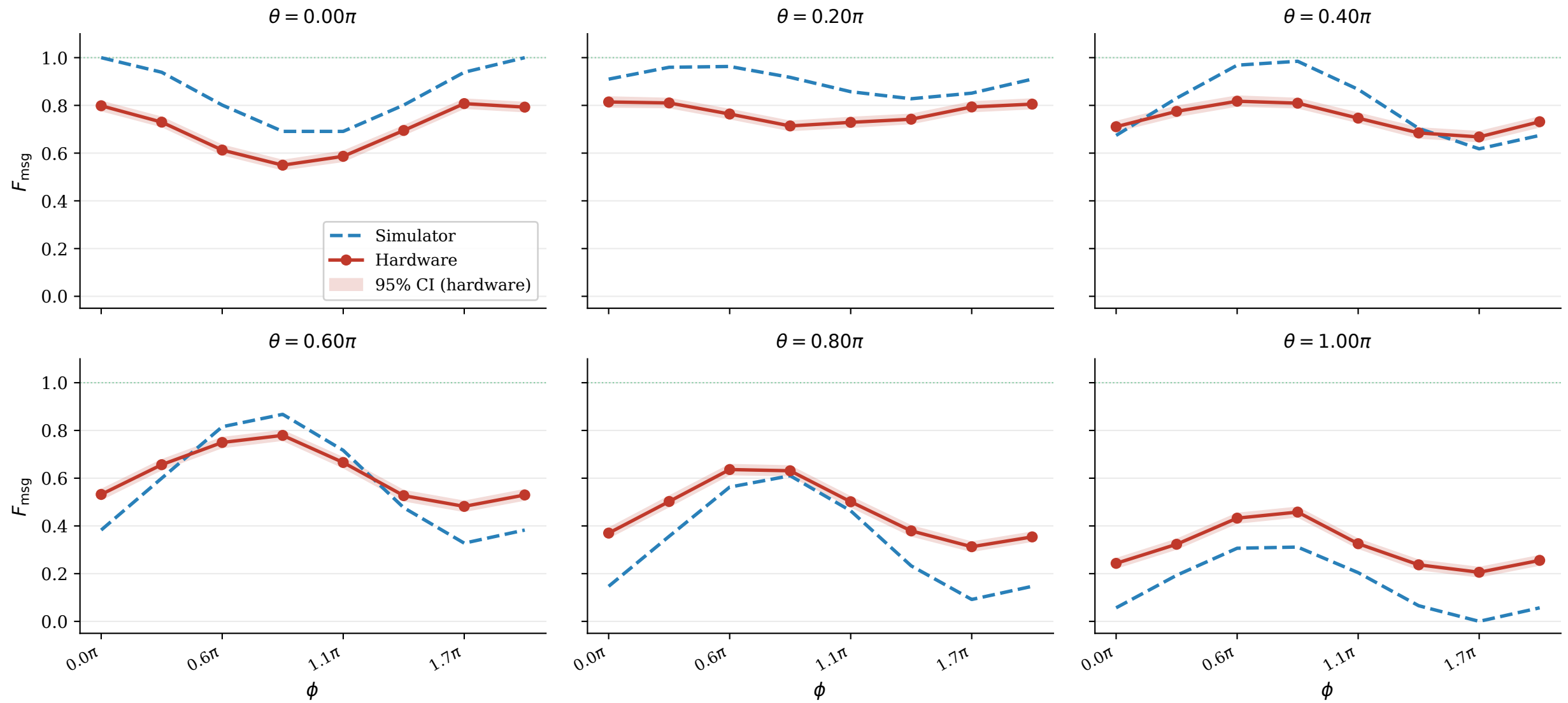
Fidelity profiles: hardware (red) vs simulator (blue dashed) Shaded band = 95% bootstrap CI on hardware
