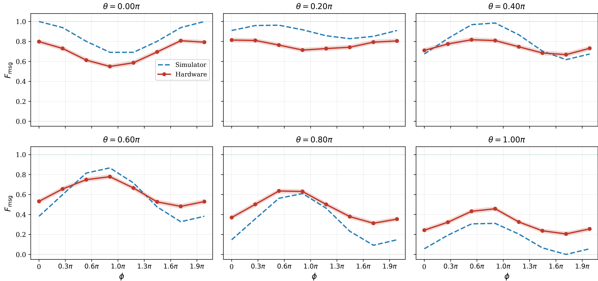
Line profiles: F_{\text{msg}}(\phi) at fixed \theta Blue dashed = simulator, Red solid = hardware \pm 95% CI ibm\_torino, 2000 shots/basis per point
