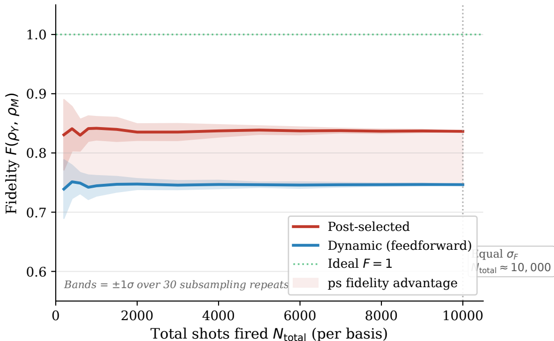
Fidelity vs. total shots fired (post-selected wastes 1 - p_{\text{succ}} \approx 76\% of shots)
