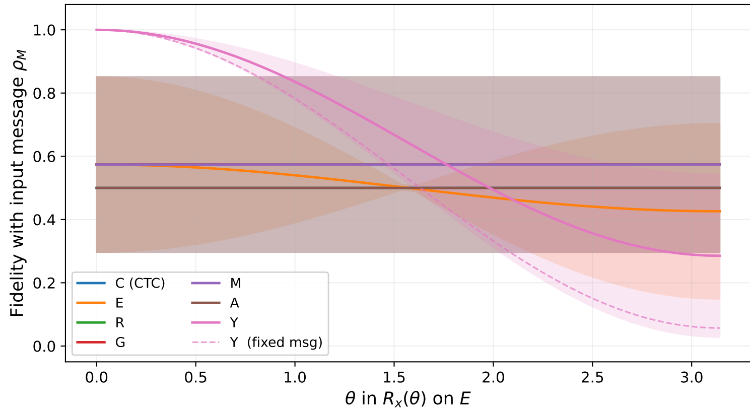
Method I: fidelity of each qubit vs \theta Mean \pm 1\sigma over 20 random message states
