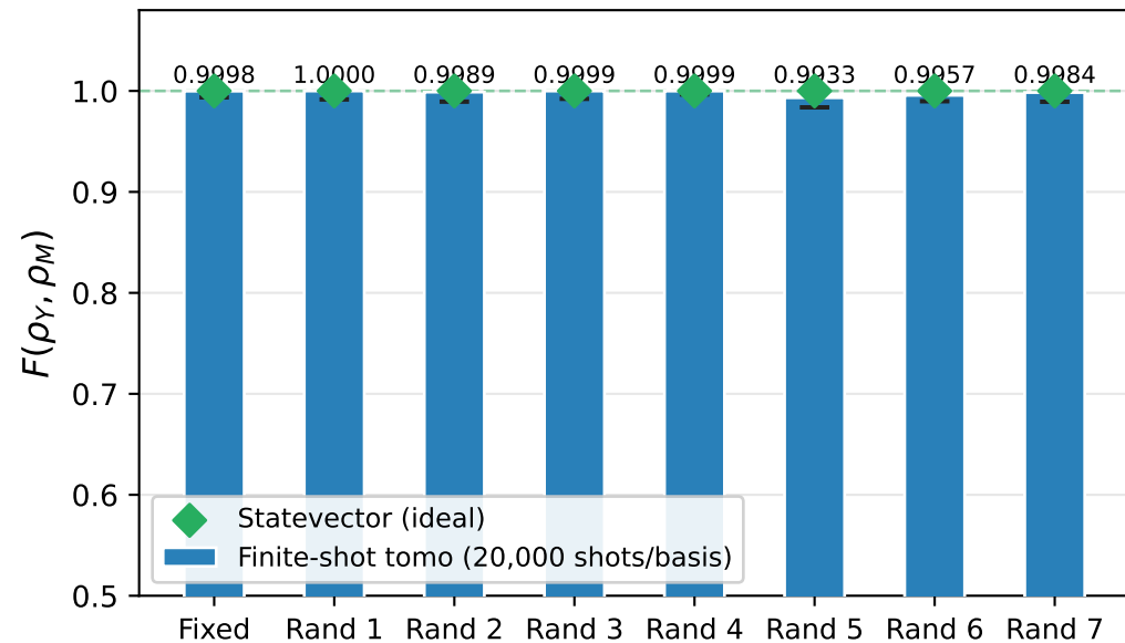
(a) Output fidelity per message state (bars = finite-shot tomo \pm 95% bootstrap CI; diamonds = statevector ideal)
