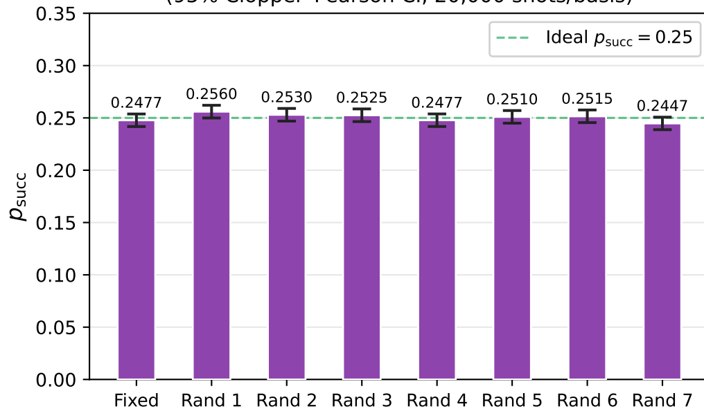
(b) Post-selection rate per message state (95% Clopper-Pearson CI, 20,000 shots/basis)
