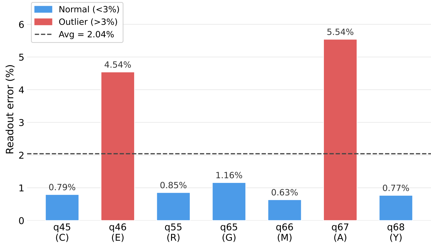
(a) ibm_torino - Readout error rates per qubit
