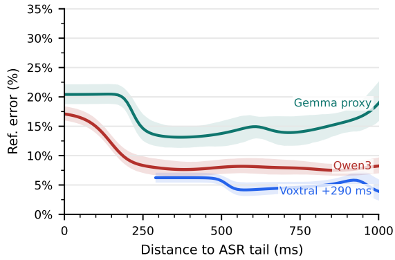
Figure 7: Live-tail ASR reference error. Reference-error rate by distance to the current ASR tail; bands are 90% audio-bootstrap intervals. Qwen3 drops from 17.1% at the tail to 8.3% at 250 ms and then stays flat. Voxtral is shifted by +290 ms CU-LongYAAL; Gemma remains unshifted because its timestamps/LongYAAL are unreliable under prompt leakage.
