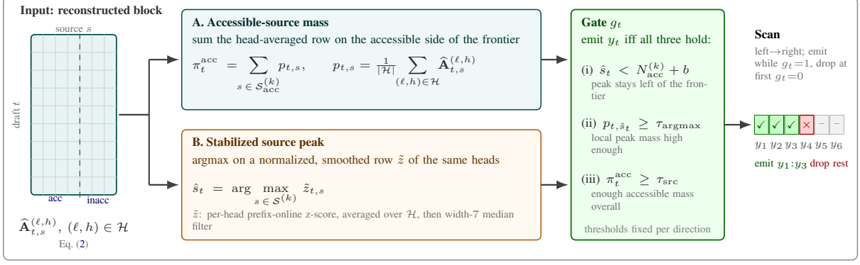
Figure 4: From the reconstructed block to an acceptance decision. The selective qk-fast reconstruction produces \hat{A}_{t,s}^{(\ell,h)} for (\ell,h) \in \mathcal{H} , with draft positions t against source positions s (left). The policy reads it through two parallel aggregations. Branch A averages the selected heads into a row p_{t,\cdot} , and sums its mass on the accessible side of the frontier, giving the provenance score \pi_t^{\text{acc}} . Branch B returns the peak \hat{s}_t of a stabilized row \tilde{z}_{t,\cdot} , where \tilde{z} is obtained by z-scoring each head with prefix-online Welford moments, averaging over \mathcal{H} , and applying a width-7 median filter along the source axis. The gate g_t accepts draft token t iff the peak stays on the accessible side of the frontier, the peak mass exceeds \tau_{\text{argmax}} , and the accessible-source mass exceeds \tau_{\text{src}} . A left-to-right scan emits the longest run of accepting tokens and drops the remainder at the first failure.
