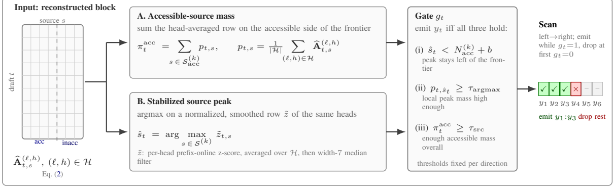
Figure 4: From the reconstructed block to an acceptance decision. The selective qk-fast reconstruction produces \hat{\mathbf{A}}_{t,s}^{(\ell,h)} for (\ell, h) \in \mathcal{H} , with draft positions t against source positions s (left). The policy reads it through two parallel aggregations. Branch A averages the selected heads into a row p_{t,\cdot} , and sums its mass on the accessible side of the frontier, giving the provenance score \pi_t^{\text{acc}} . Branch B returns the peak \hat{s}_t of a stabilized row \tilde{z}_{t,\cdot} , where \tilde{z} is obtained by z-scoring each head with prefix-online Welford moments, averaging over \mathcal{H} , and applying a width-7 median filter along the source axis. The gate g_t accepts draft token t iff the peak stays on the accessible side of the frontier, the peak mass exceeds \tau_{\text{argmax}} , and the accessible-source mass exceeds \tau_{\text{src}} . A left-to-right scan emits the longest run of accepting tokens and drops the remainder at the first failure.
