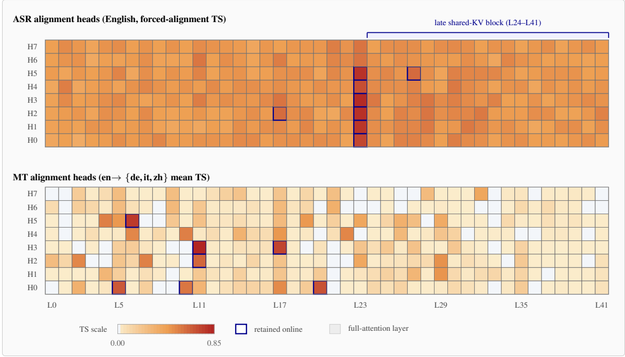
Figure 8: Architecture-aware view of Gemma AlignAtt heads. Each heatmap covers Gemma’s 42 layers (horizontal axis) and 8 query heads (vertical axis); color encodes mean token-alignment score TS on a shared [0, \max] scale, so empty cells read as low rather than “below threshold”. Top: audio-to-text alignment heads, scored by forced-alignment MAE on English dev audio. Bottom: source-to-target translation heads, averaged over \text{en} \rightarrow \{\text{de}, \text{it}, \text{zh}\} . Blue outlines mark the per-role retained heads ( \mathcal{H}_{\text{ASR}} and \mathcal{H}_{\text{MT}} ); grey vertical stripes mark full-attention layers; the blue bracket delimits the late shared-KV block, where observer cost follows KV-group ownership rather than query-head count. The two retained sets concentrate in disjoint depth regions, consistent with per-role functional specialization.
