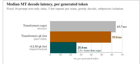
Figure 6: Inference-time comparison of MT capture seams. Median latency per generated token on a fixed 16-prompt text-only suite, for a minimal Transformers eager reference, a Transformers qk-fast reference that reconstructs source rows from captured layer inputs, and the engine-native vLLM qk-fast path used by the shipped backend. Each seam uses one unmeasured warmup pass followed by three hot repeats, greedy decode, a fixed AlignAtt head set, and subprocess isolation; per-prompt results and divergences are stored in the generated JSON artifact.
