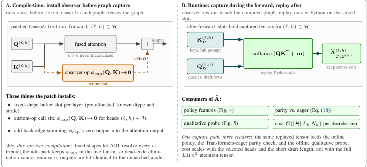
Figure 9: Compile-safe observer lifecycle on the deployed vLLM path. Left (A), once, before graph capture: the forward of GemmaAttention is patched so that for each selected head (\ell, h) \in \mathcal{H} the query and key tensors also pass through an observer custom op \phi_{\text{cap}} (dashed orange side path). The op writes the selected slices into fixed-shape, pre-allocated slots and returns a zero tensor that is added back into the attention output; this keeps the op in the live fan-in of the graph so the compiler cannot dead-code-eliminate it, while the numerical output of the layer is unchanged. Right (B), every forward: after the compiled forward finishes, the observer slots hold \mathbf{K}_P^{(\ell, h)} for the full prompt and \mathbf{Q}_D^{(\ell, h)} for the draft rows; a short Python-side replay computes \mathbf{Q}\mathbf{K}^\top for the draft against the full prompt, applies the causal mask \mathbf{m} , takes the softmax, and keeps the source columns to yield the selective block \hat{\mathbf{A}}_{D, S^{(k)}}^{(\ell, h)} that feeds the policy, the parity check against an uncompiled Transformers reference, and the qualitative probe.
