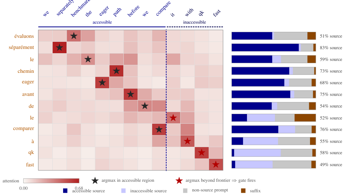
Figure 5: Word-level selective reconstruction on a live MT draft. Top ribbon: the decoder-only prompt is split into the system instruction, the live source (with the accessibility frontier shown in-line between the committed accessible prefix and the still-inaccessible tail), the already accepted target prefix reused from earlier streaming steps, and the draft currently under inference. Left panel: reconstructed draft-to-source attention from the selected AlignAtt heads, aggregated to the word level; rows are drafted words, columns are source words split by the dashed frontier. A star marks the per-row argmax (black when it lands in the accessible region, red when it lands beyond the frontier, which is exactly what triggers the SOURCE-FRONTIER gate). Right panel: for each drafted word the reconstructed attention mass is partitioned into the four provenance classes; the numeric annotation is the total source share (accessible + inaccessible). The green band is previously committed target text reused as causal context; it is not itself the object of the gate. The first black stars in the orange draft show that newly proposed words may still align to multiple source words inside the current accessible span, and only the first red star beyond the frontier triggers rejection.
