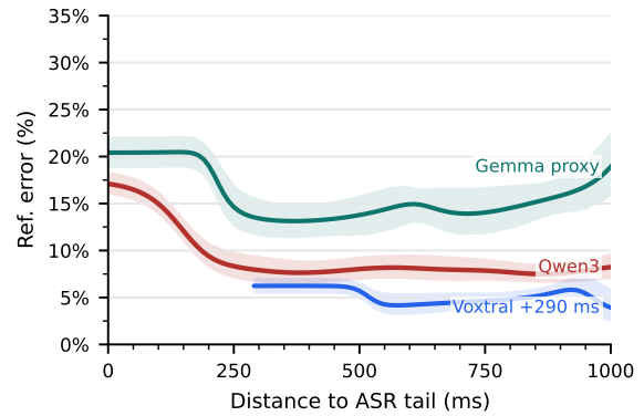
Figure 7: Live-tail ASR reference error . Reference-error rate by distance to the current ASR tail; bands are 90% audio-bootstrap intervals. Qwen3 drops from 17.1% at the tail to 8.3% at 250 ms and then stays flat. Voxtral is shifted by +290 ms CU-LongYAAL; Gemma remains unshifted because its timestamps/LongYAAL are unreliable under prompt leakage.
