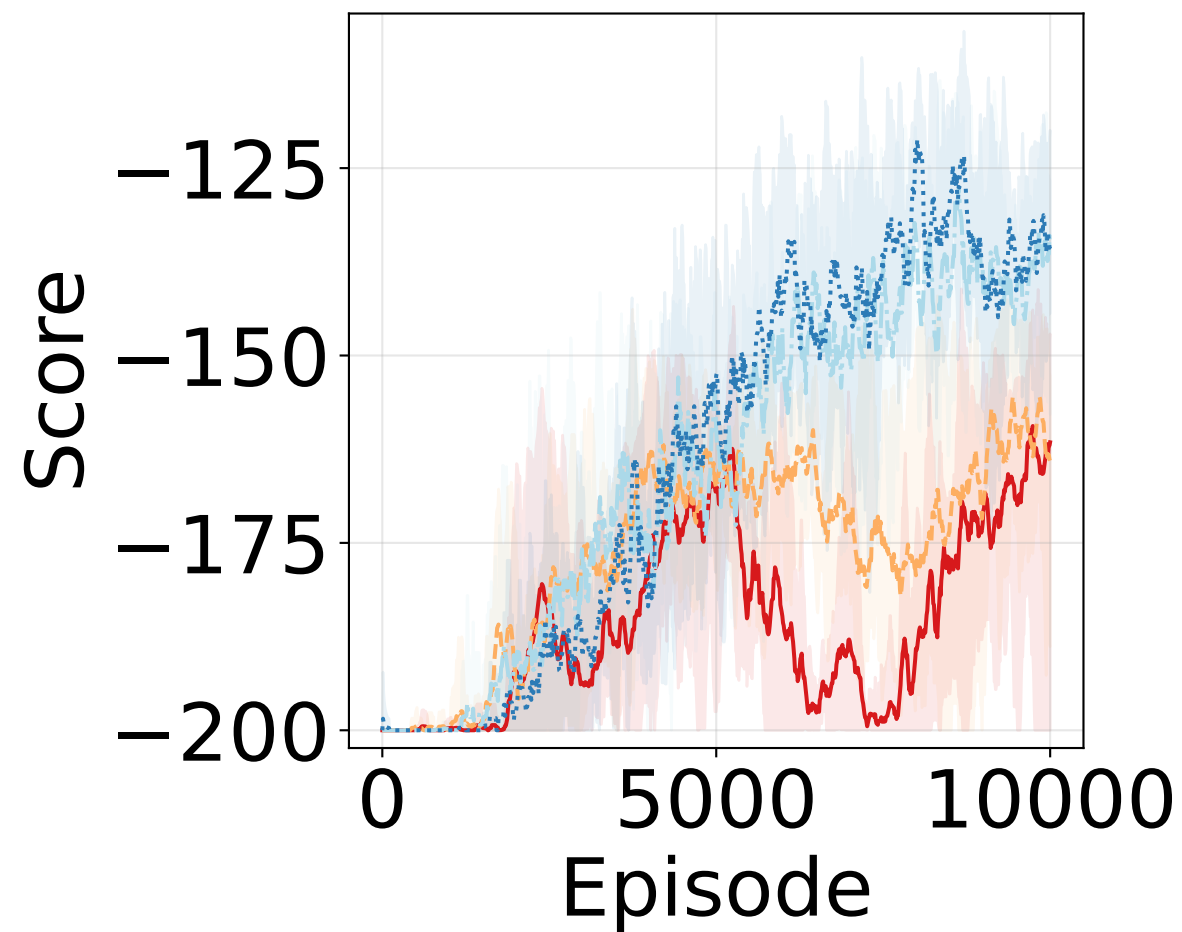
MountainCar-v0
