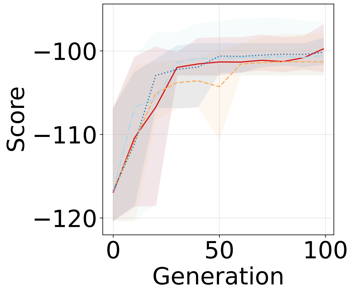
MountainCar-v0
