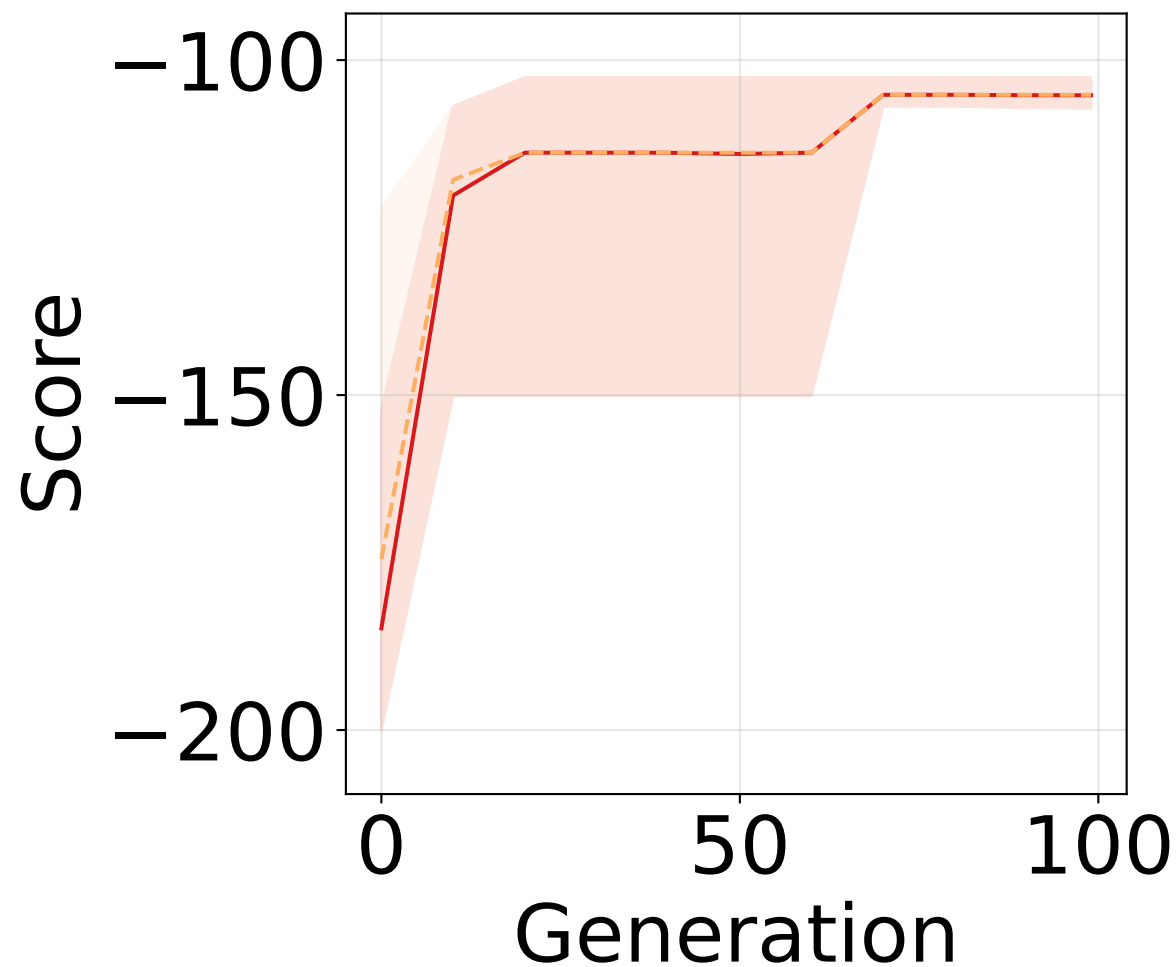
MountainCar-v0
