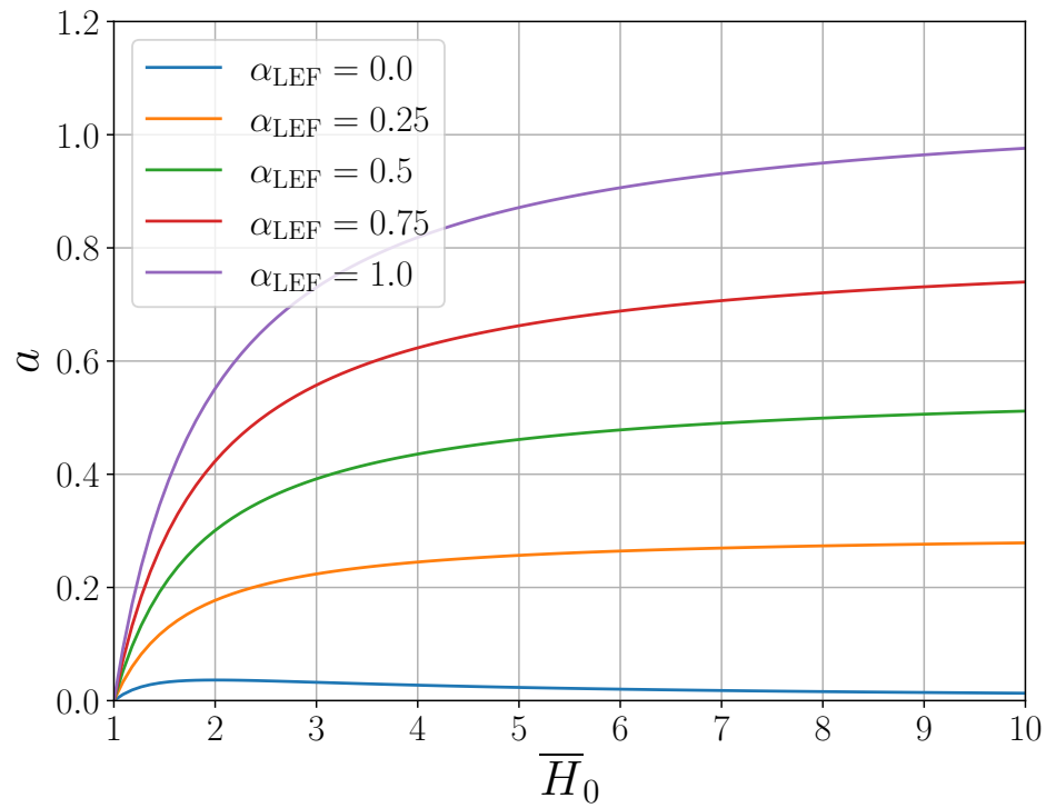
Figure 7.6: Approximate analytic solution for the mean-field quadratic decay coefficient given by Eq. (7.166b) as a function of \bar{H}_0 for various linewidth enhancement factors. Here D_2 = 1.5 \times 10^{-5} .
