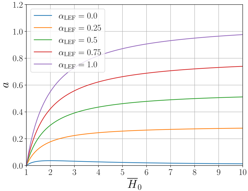
Figure 7.6: Approximate analytic solution for the mean-field quadratic decay coefficient given by Eq. (7.170b) as a function of \bar{H}_0 for various linewidth enhancement factors. Here D_2 = 1.5 \times 10^{-5} .
