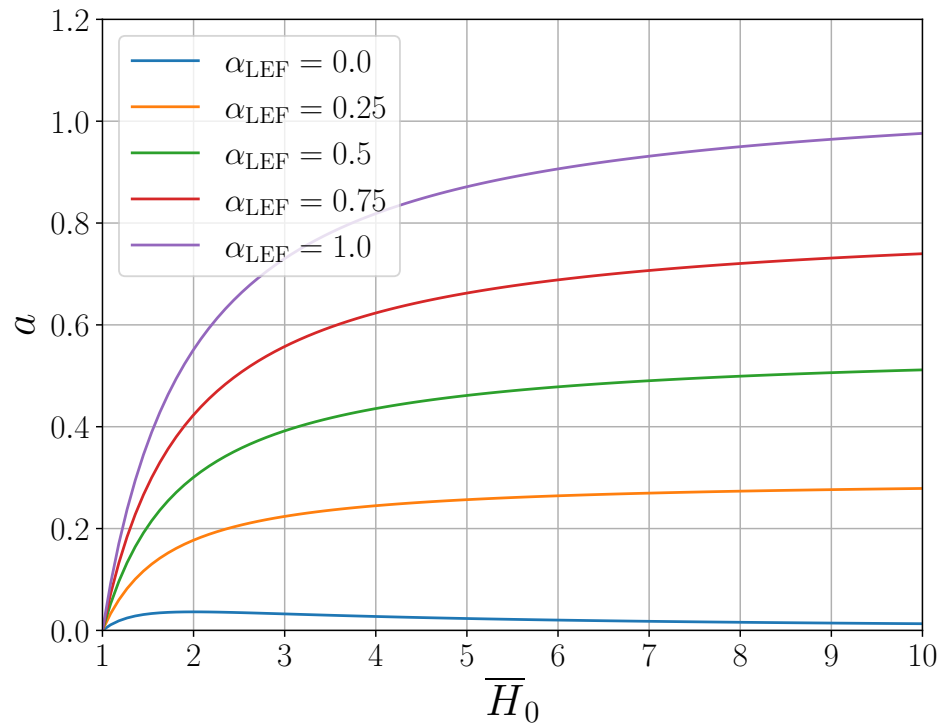
Figure 7.6: Approximate analytic solution for the mean-field quadratic decay coefficient given by Eq. (7.162b) as a function of \bar{H}_0 for various linewidth enhancement factors. Here D_2 = 1.5 \times 10^{-5} .
