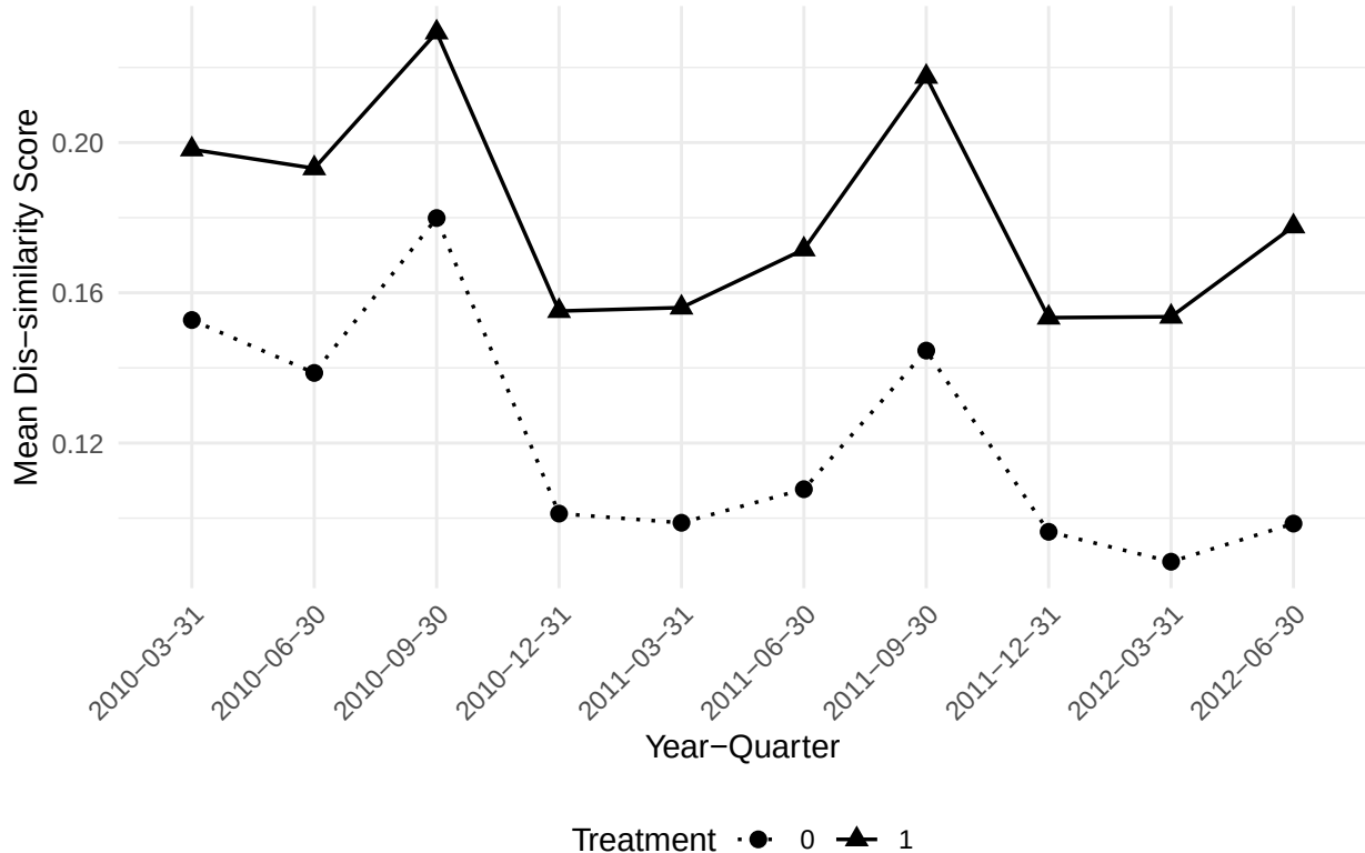
Dis-similarity Trends by Treatment Group
