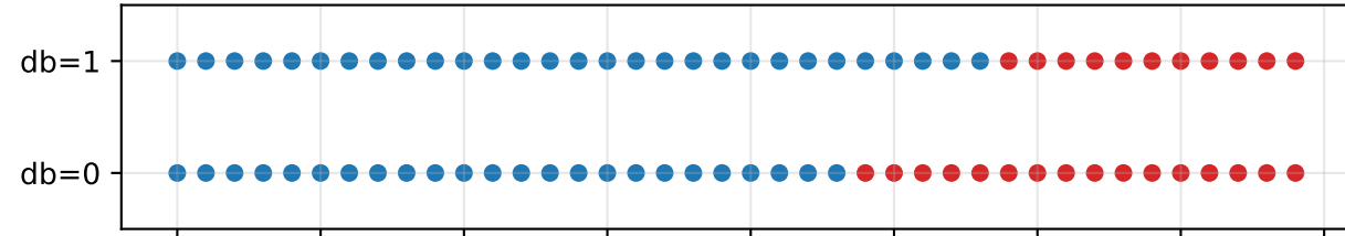
N=3 | Siegert FP enumeration | J(db=0)=0.00, J(db=1)=0.27
