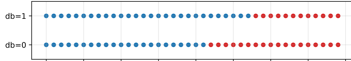
N=4 | Siegert FP enumeration | J(db=0)=0.00, J(db=1)=0.10
