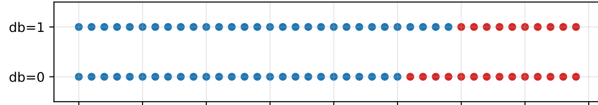
N=2 | Siegert FP enumeration | J(db=0)=0.00, J(db=1)=0.29
