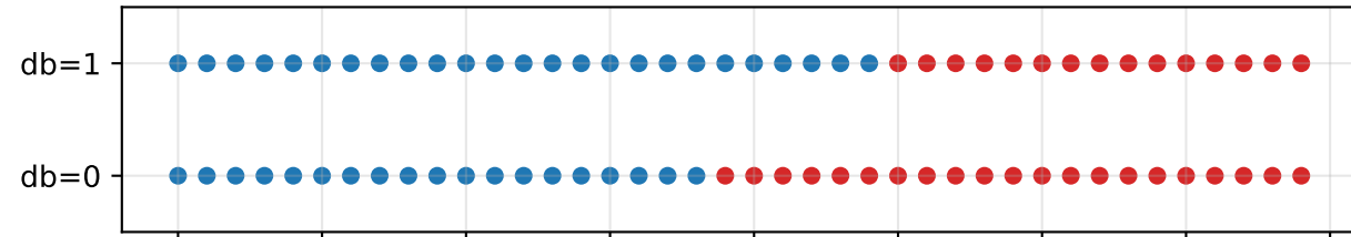
N=6 | Siegert FP enumeration | J(db=0)=0.00, J(db=1)=0.14
