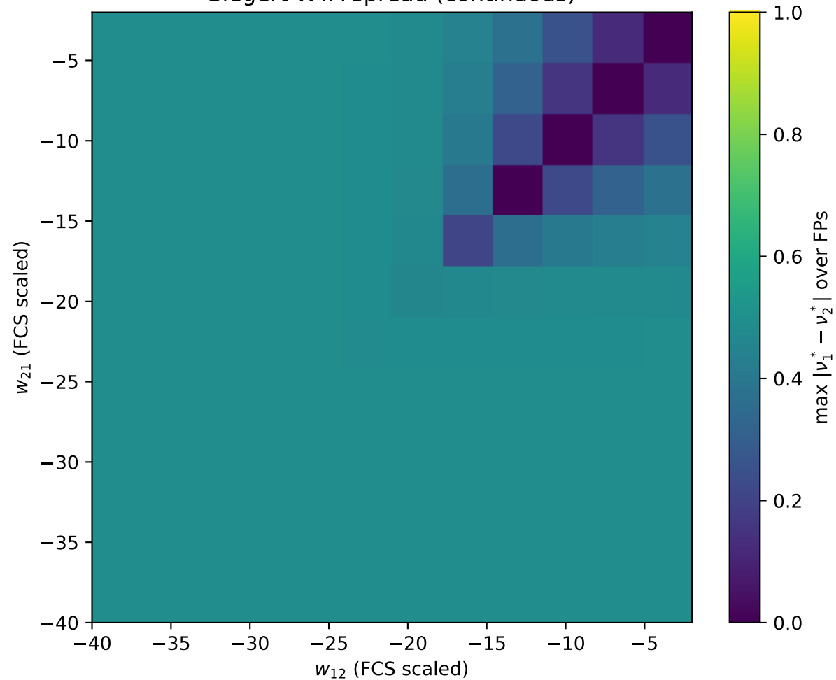
Siebert WTA spread (continuous)
