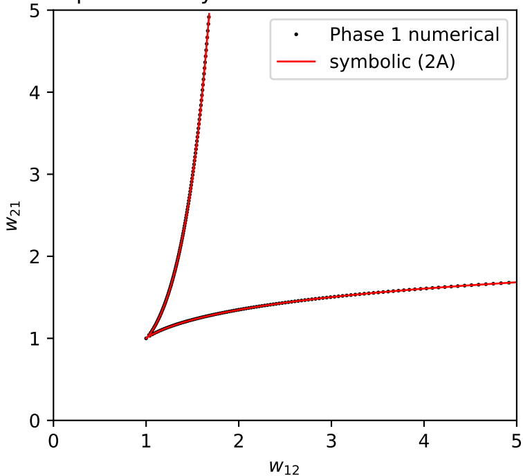
2A pitchfork: symbolic vs Phase 1 numerical
