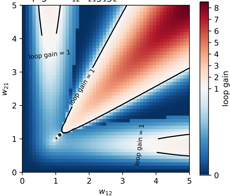
Loop gain w_{12}w_{21}g_1g_2 at the saddle FP
