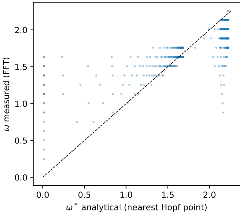
Oscillation frequency: analytical vs measured
