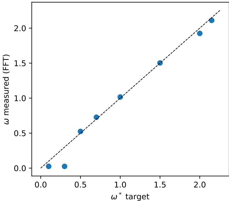
Pole placement: target vs realised frequency
