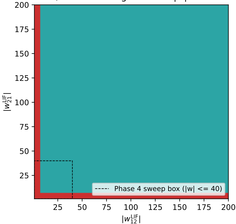
LI\&F bistable region out to |w| \leq 200
