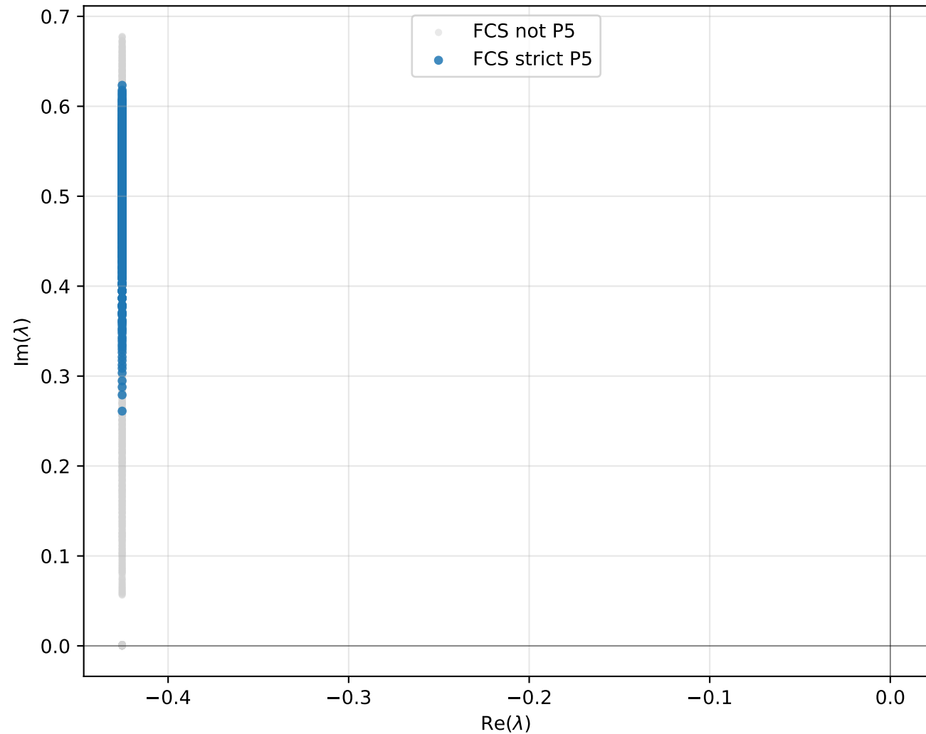
Phase 1: Jacobian eigenvalue spectrum across grid ( \text{Re} = -1/\tau_m = -0.425 for all complex cells)
