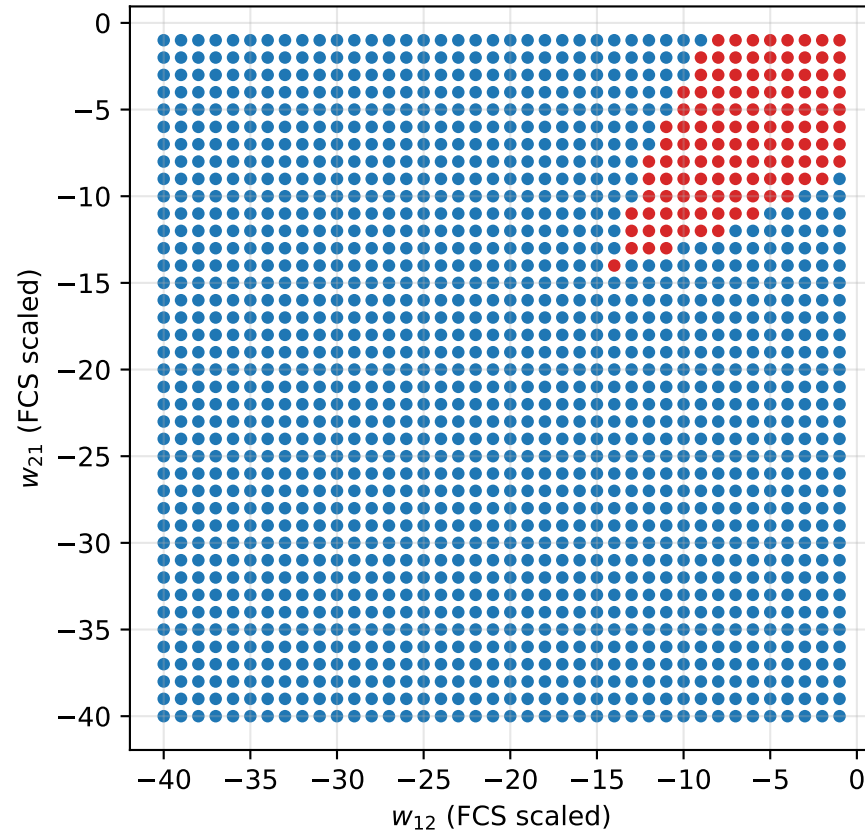
Phase 1: Siegert (static) reading of FCS Property 7 Siegert FP enumeration 1482/1600 blue Jaccard vs FCS = 0.680
