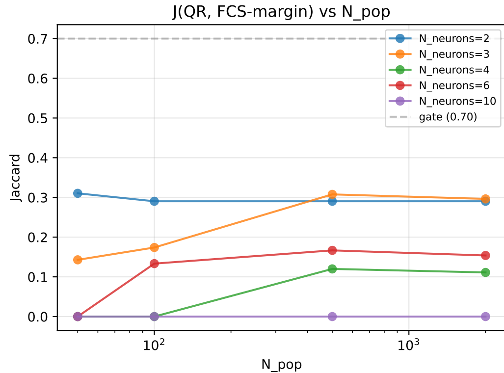
Phase 3 Jaccard curves vs N_pop
