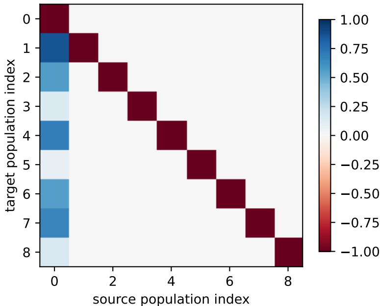
5B: Jacobian of parallel composition (n=8)
