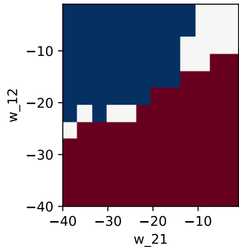
Quasi-renewal N = 100
