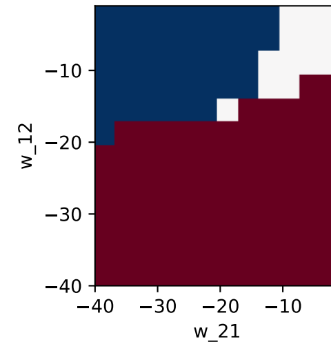
Quasi-renewal N = 2000
