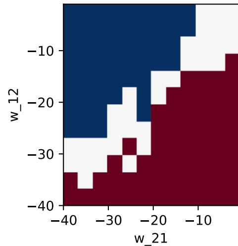
Quasi-renewal N = 50
