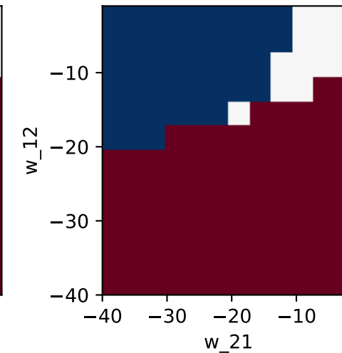
Quasi-renewal N = 500
