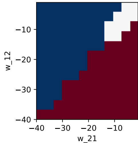
Siegert mean-field
