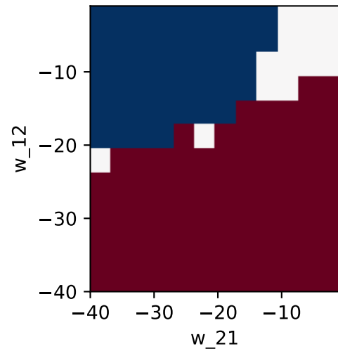
Quasi-renewal N = 200
