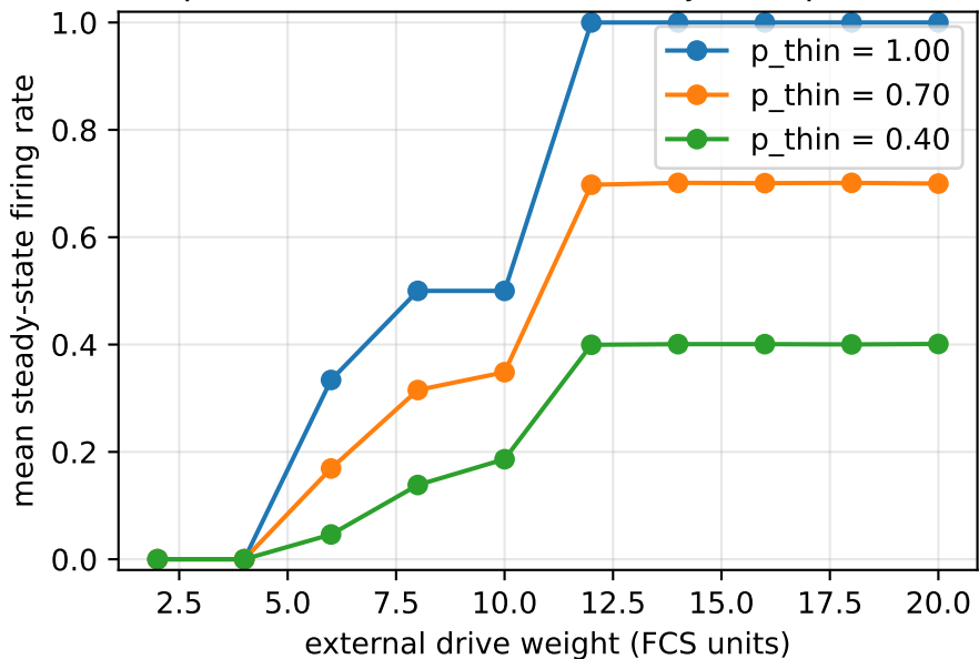
V0.1 Population f-I curve (threshold jitter eps=2, N=100)
