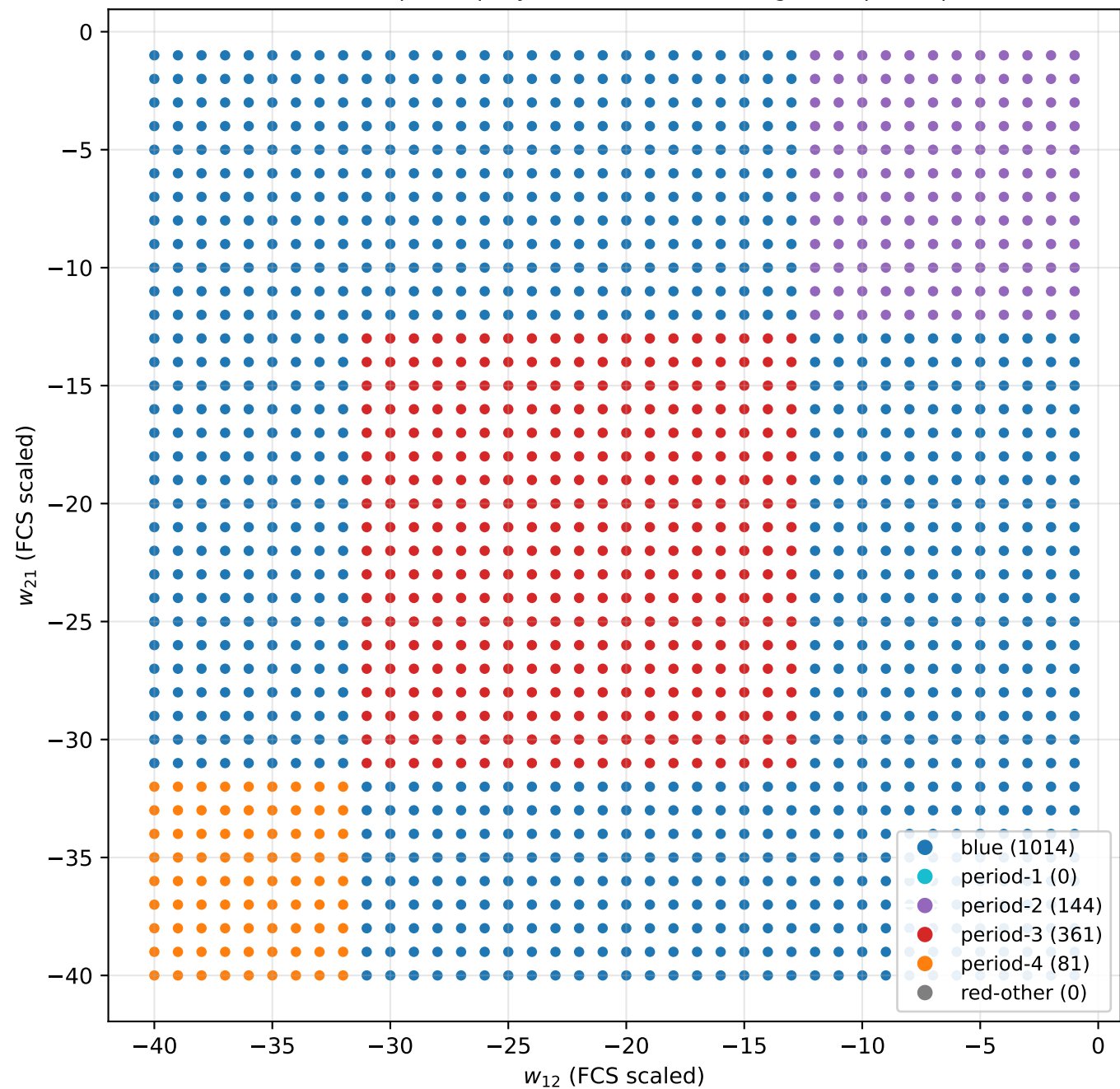
Per-cell synchrony classification of FCS Property 7 grid (blue: WTA; period-p: synchronous lock at integer-tick period p)
