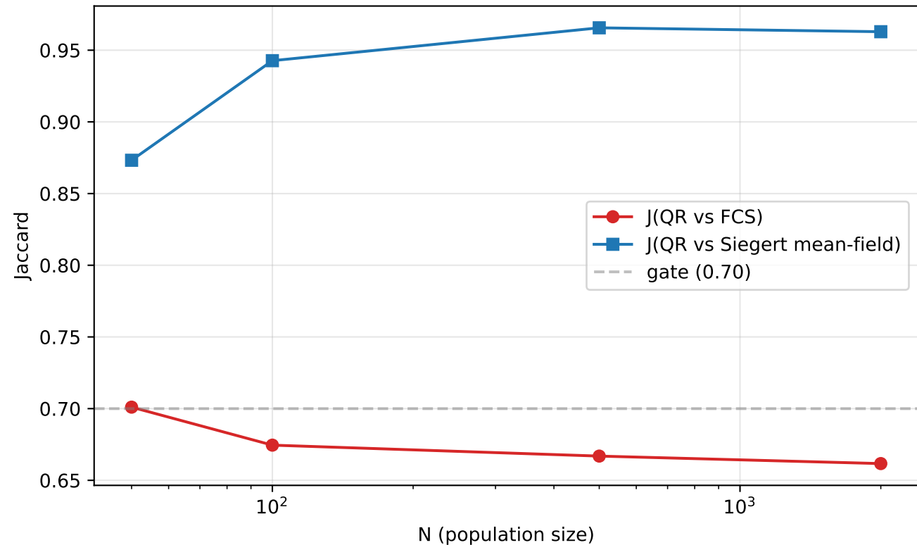
QR Jaccard vs FCS and Siegert across N
