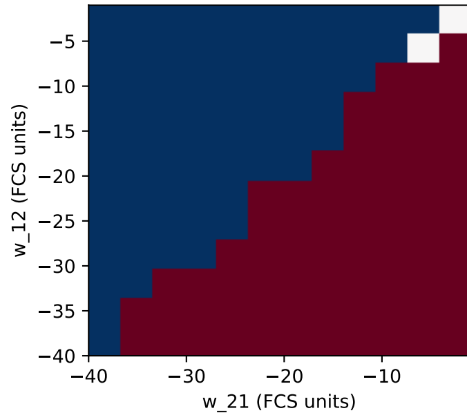
Population thread (sigmoid)
