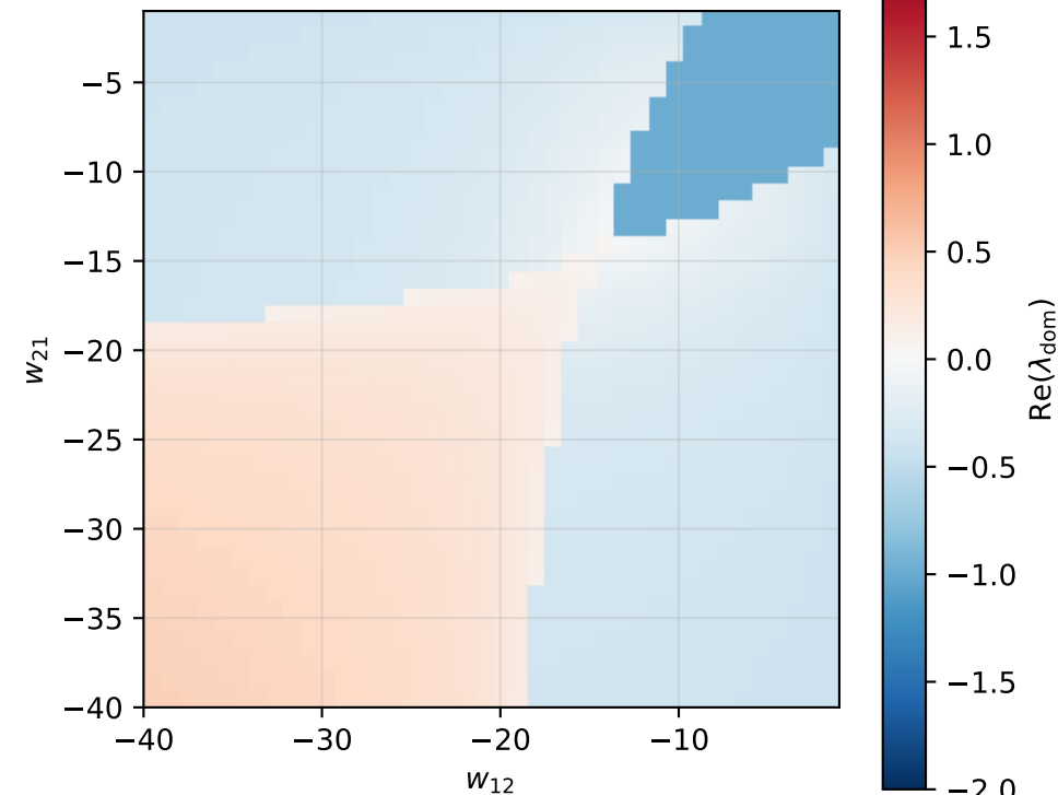
\text{Re}(\lambda_{\text{dom}}) (clipped to \pm 2 )
