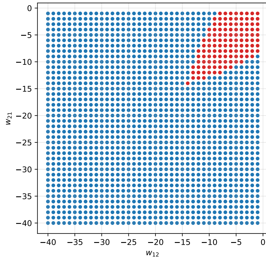
Phase 1: Siebert FP 1482/1600 blue, J=0.680
