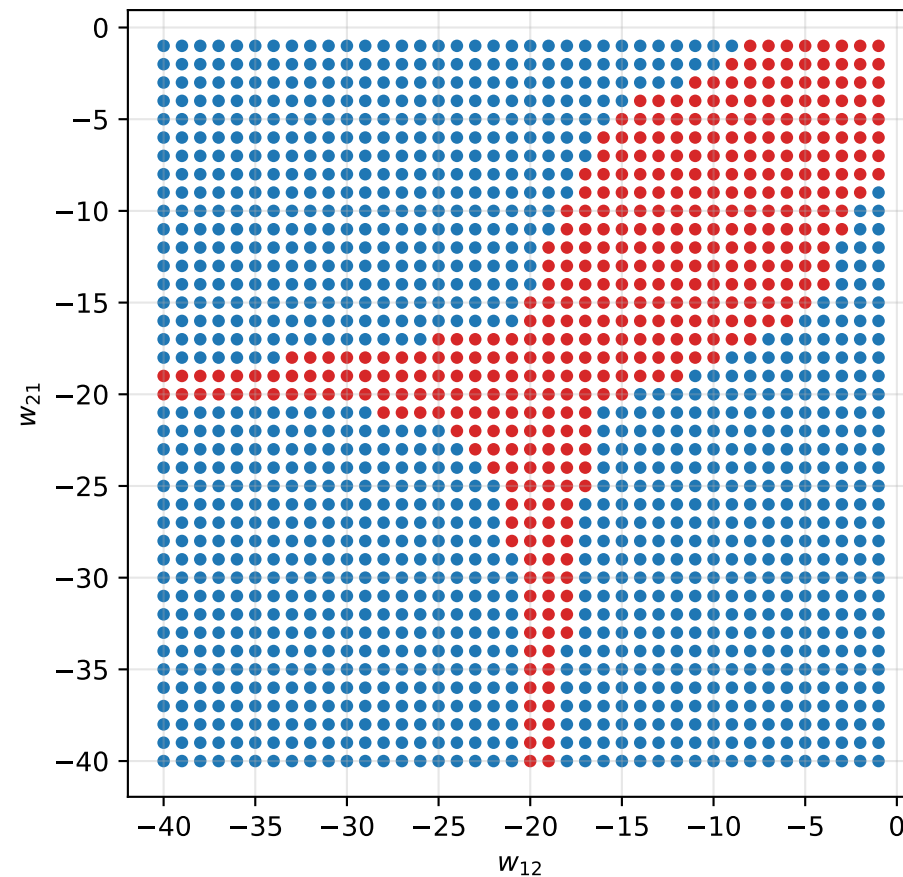
Phase 2: H(\omega) eigenvalue gate vs FCS Property 7 Phase 2: |\text{Re}(\lambda)| > 0.25 gate 1191/1600 blue, J=0.677
