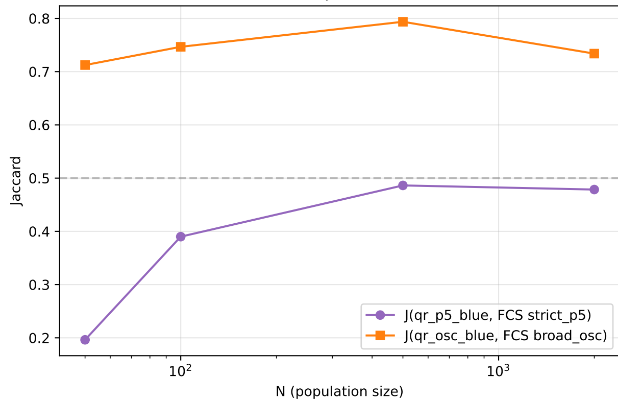
Phase 3 Jaccard vs N
