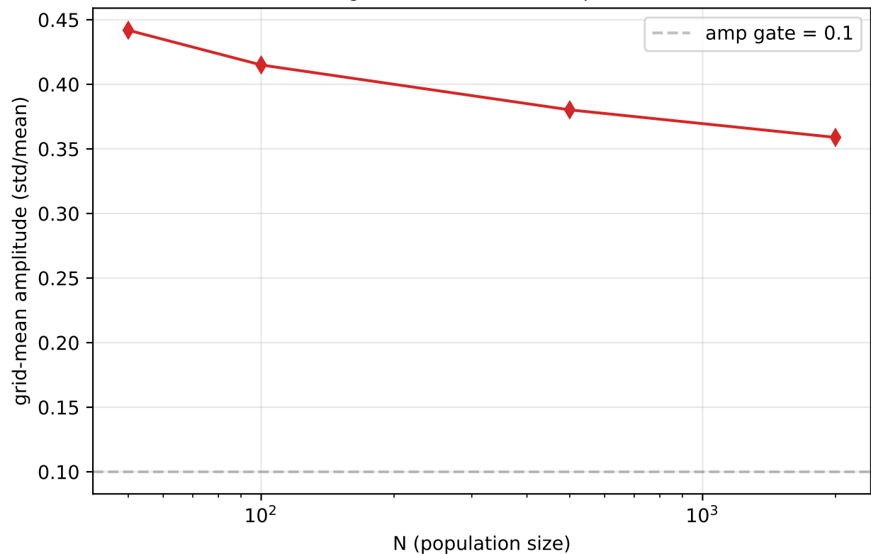
Phase 3 grid-mean oscillation amplitude vs N
