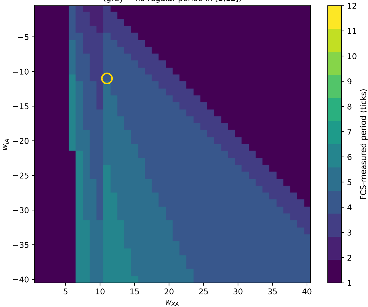
Phase 0: FCS-measured period of A on negative-loop grid (grey = no regular period in [2,12])
