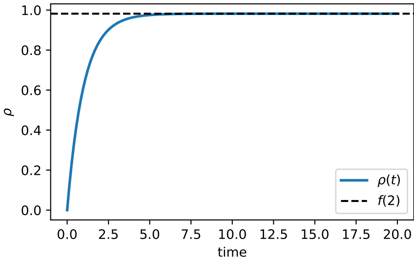
V0.1 single population converging to f(l)
