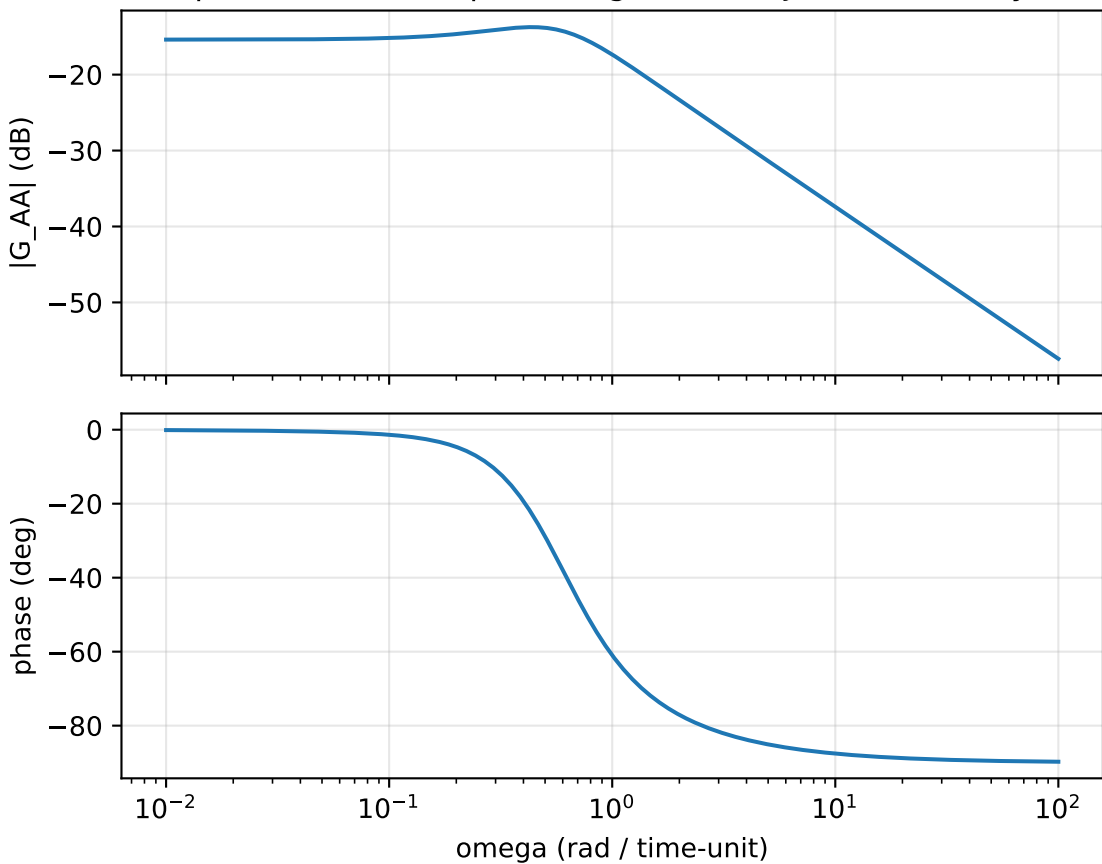
Bode plot of closed-loop G(\omega) = (I - HJ)^{-1} H , entry A→A
