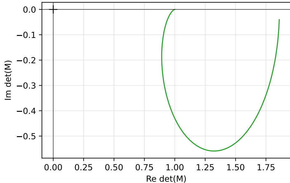
Nyquist locus of \det(M(\omega))
