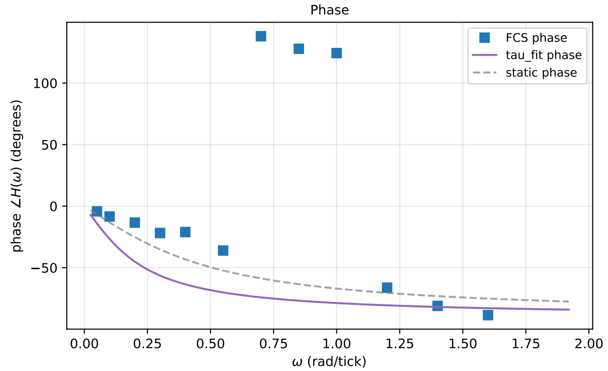
Experiment A: Bode response of isolated FCS neuron, single-pole fit
