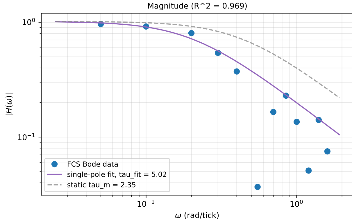
Experiment A: Bode response of isolated FCS neuron, single-pole fit
