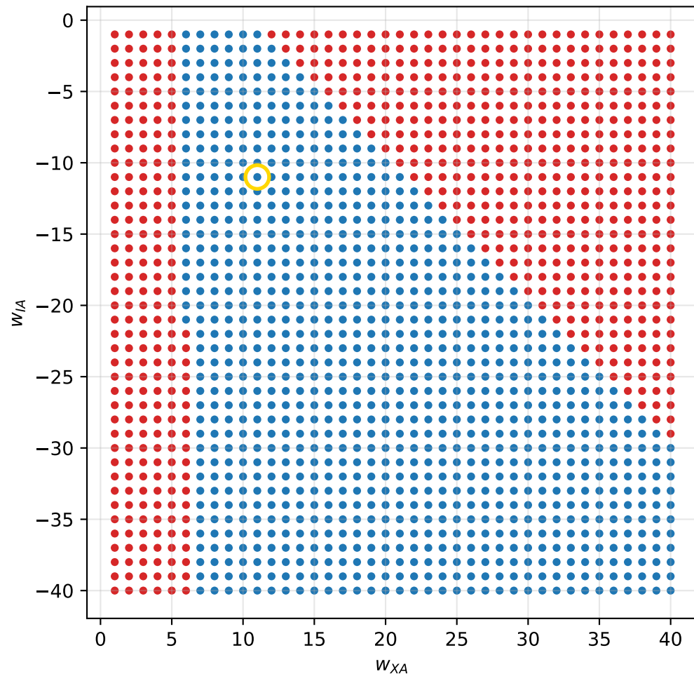
Phase 1: Siegert FP + Jacobian vs FCS Property 5 FCS broad oscillation 946/1600 blue
