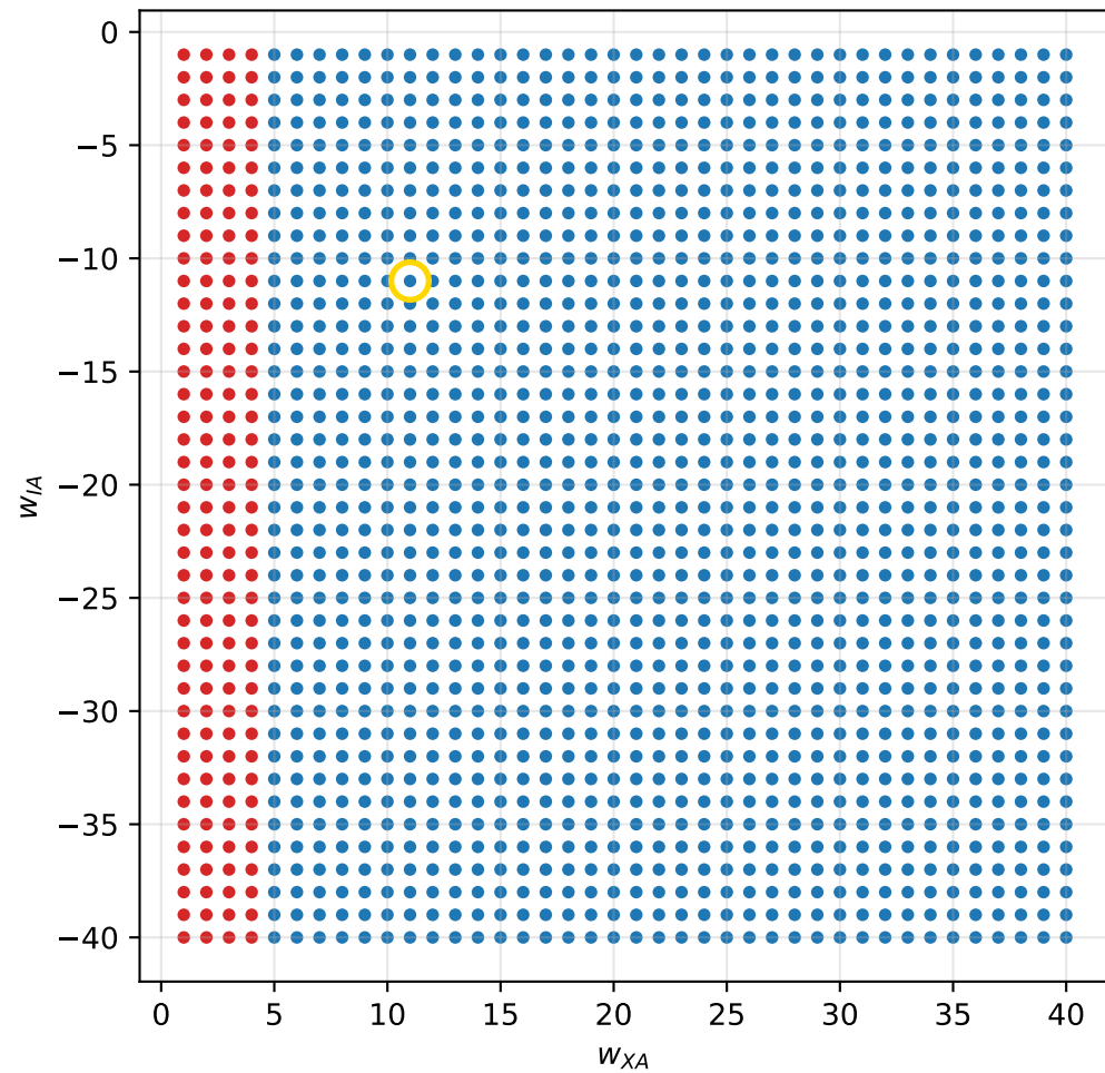
Siegert spiral ( \text{Im}(\lambda) \neq 0 ) 1440/1600 blue J(\text{strict})=0.309 , J(\text{broad})=0.657
