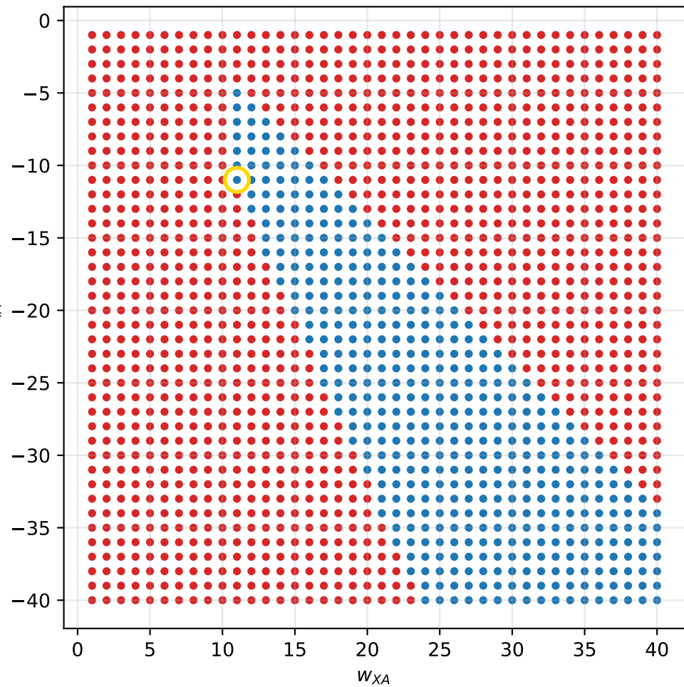
FCS strict Property 5 445/1600 blue
