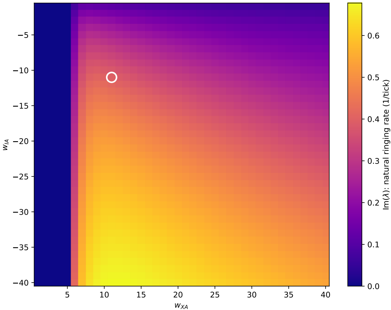
Phase 1: \text{Im}(\lambda) heatmap — predicted ringing frequency at the FP
