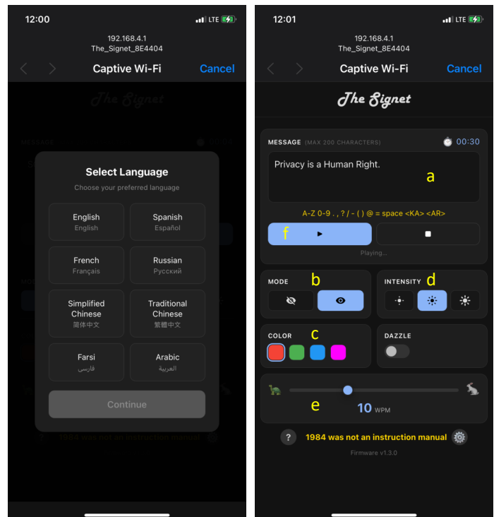
iPhone UI examples
